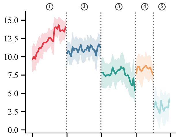
Mean Reward
